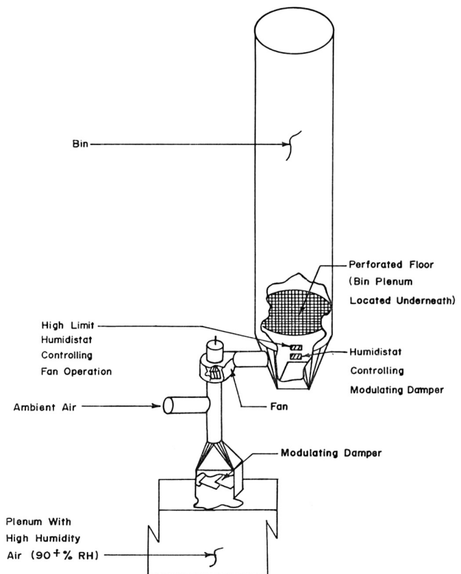
Fig. 1. Schematic of one of the humidity controlled bins used to aerate the Spanish peanuts.
