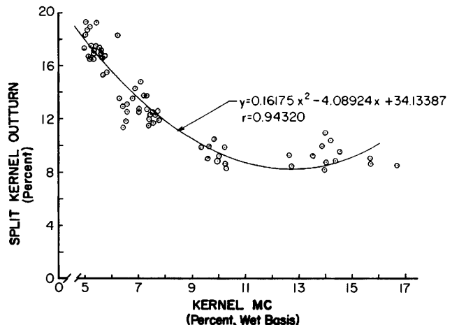
Fig. 3. The effect of kernel remoisturizing on the percent split kernel outturn for the Virginia peanuts.
